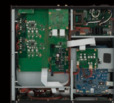
Internal configuration (Bottom side)
