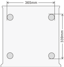
Insulator position / dimensions
